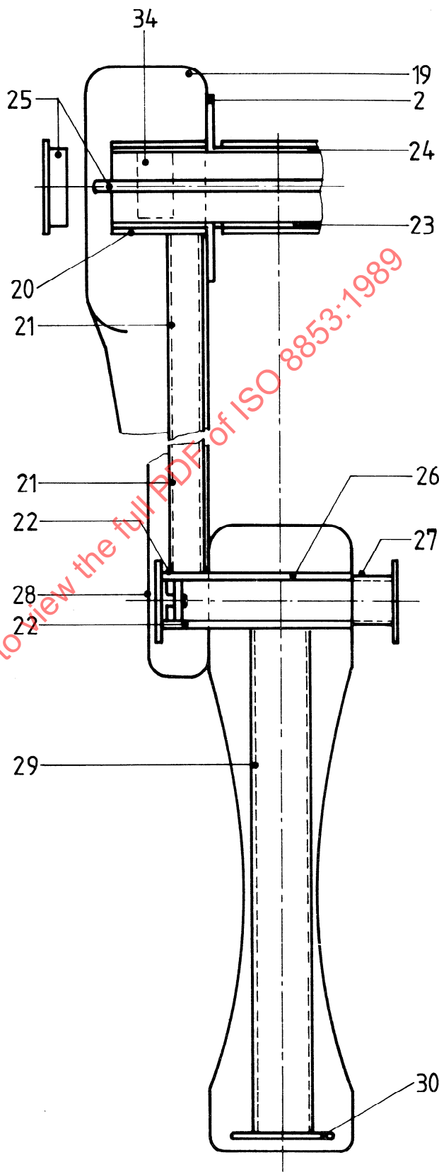
Figure B.4 — Hip, thigh and lower leg — Front view
