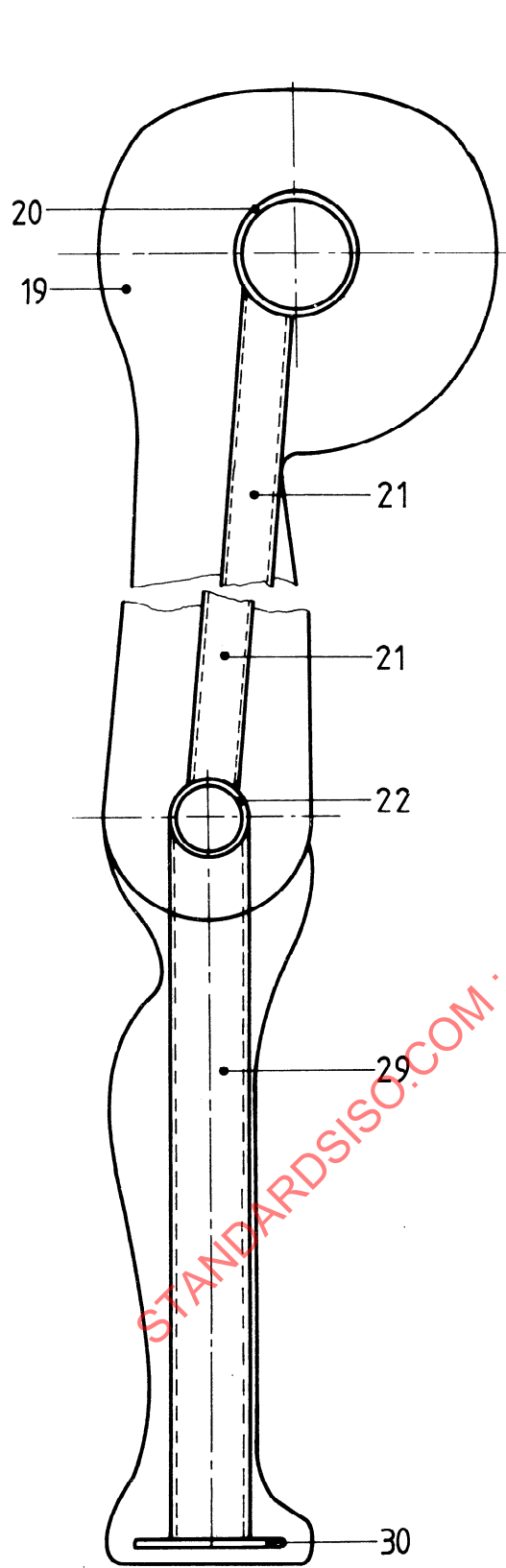
Figure B.3 — Hip, thigh and lower leg — Side view
