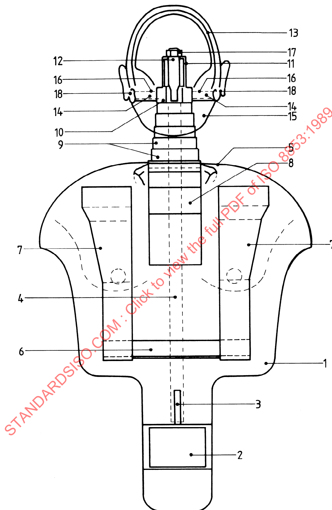
Figure B.2 — Head, neck and body — Front view
