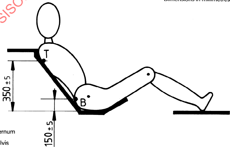
Figure B.6 — Measuring points for movement of a seated manikin
