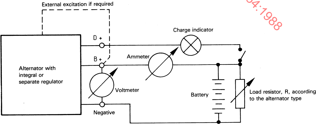
Figure 1 — Diagram for alternator testing
