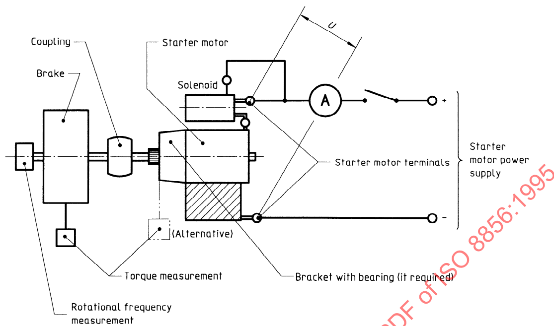
Figure 3 — Type 2 test bench
