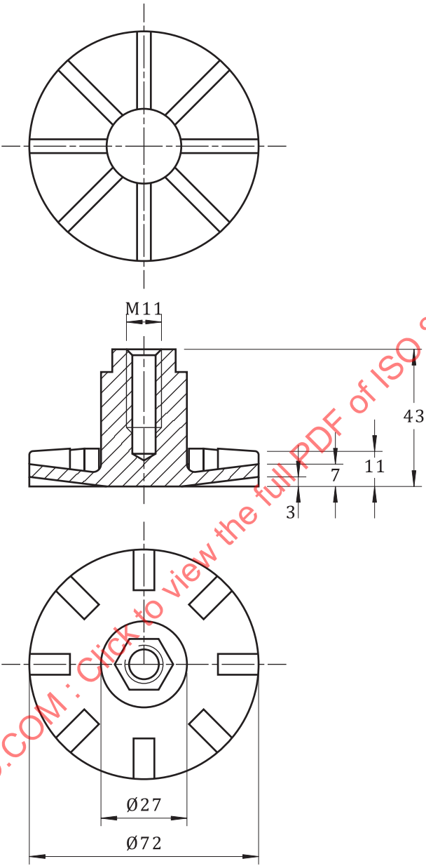
Figure 5 — Impeller
