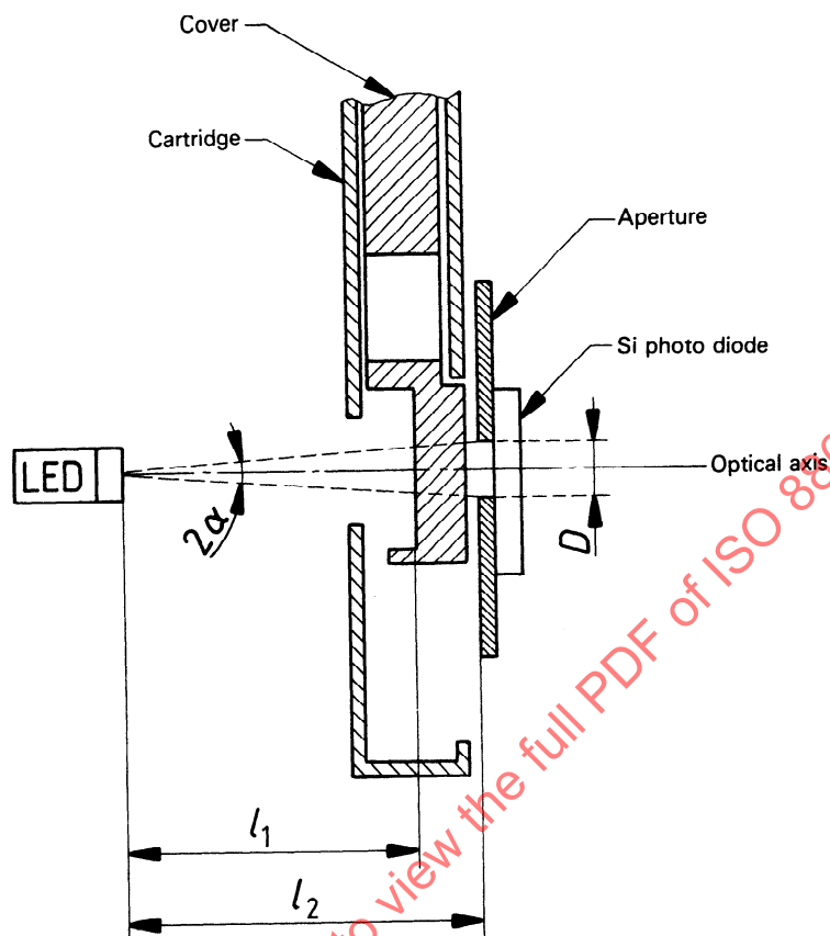
Figure 9 — Measuring device
