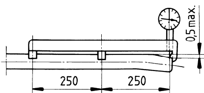
Figure 1 — Measuring tube end curvature
