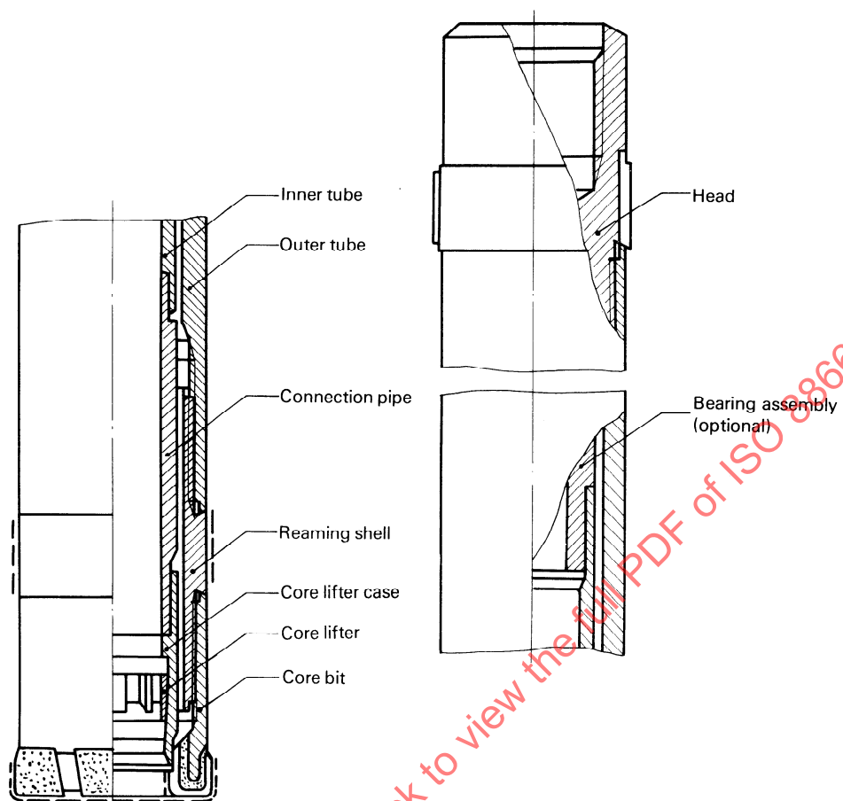
Figure 29 — Assembly of double-tube core barrel, type DP
