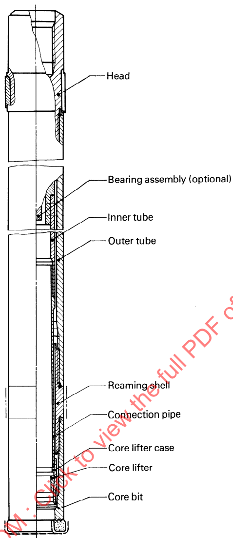
Figure 20 — Assembly of double-tube core barrel, type DM
