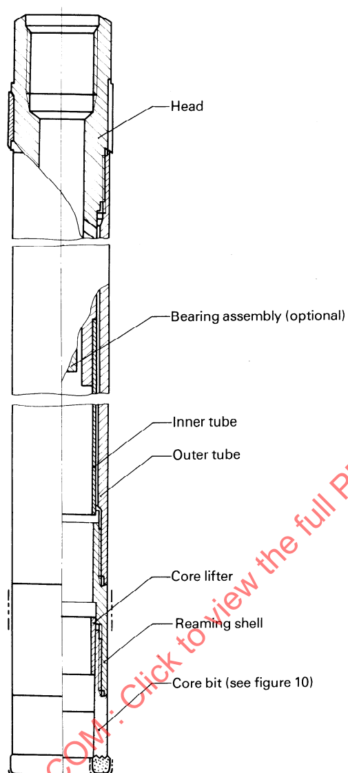
Figure 15 — Assembly of double-tube core barrel, type DM
