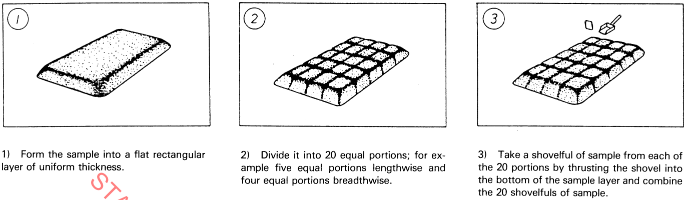
Figure 2 — Example of manual increment division for a gross sample
