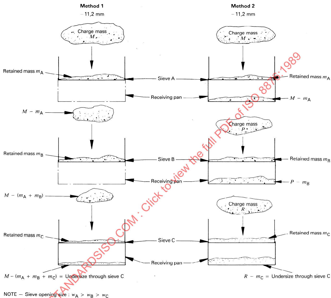
Figure 2 — Examples of alternative methods for use of individual sieves for fluorspar of particle size - 11,2 mm, + 1 mm
