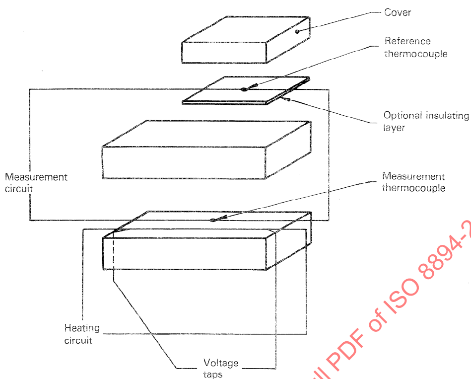
Figure 1 — Diagram showing location of heating circuit and measurement circuit (differential thermocouple circuit)
