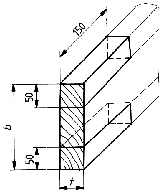
Figure 1 — Test pieces
