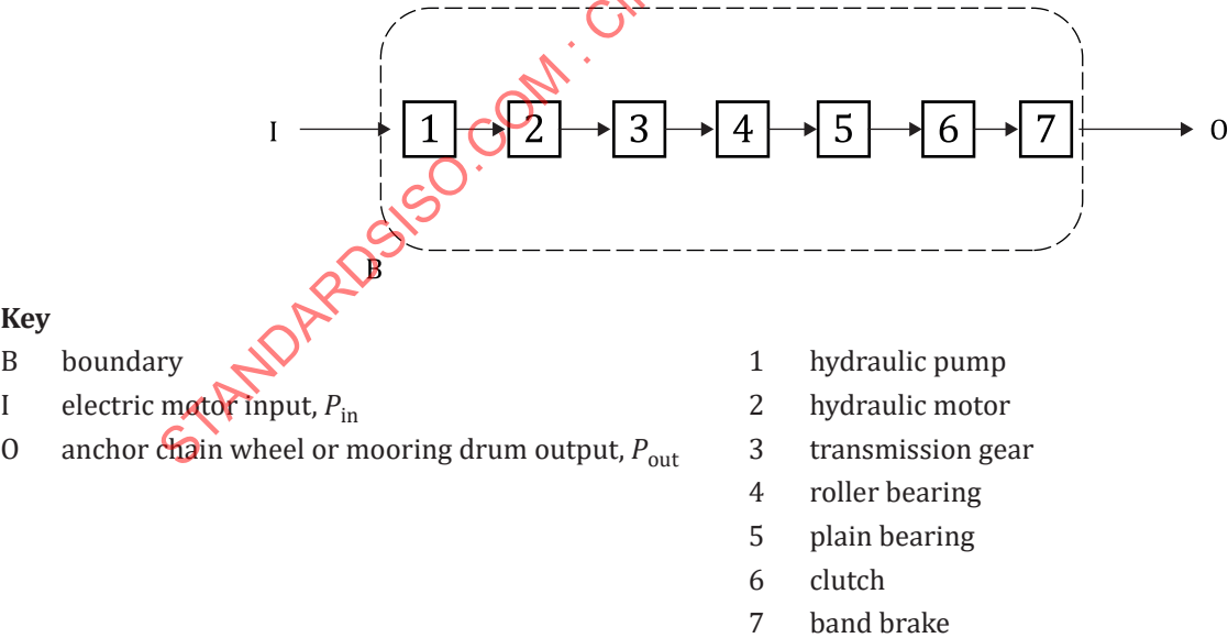
Figure 9.4 — Composition of anchor and mooring winch system
