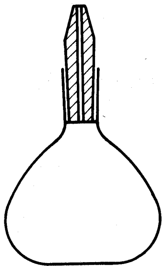
Figure 1 — Gay-Lussac pyknometer
