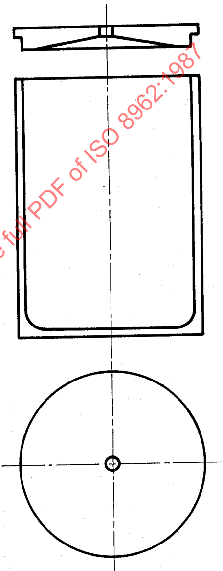
Figure 3 — Metal pyknometer
