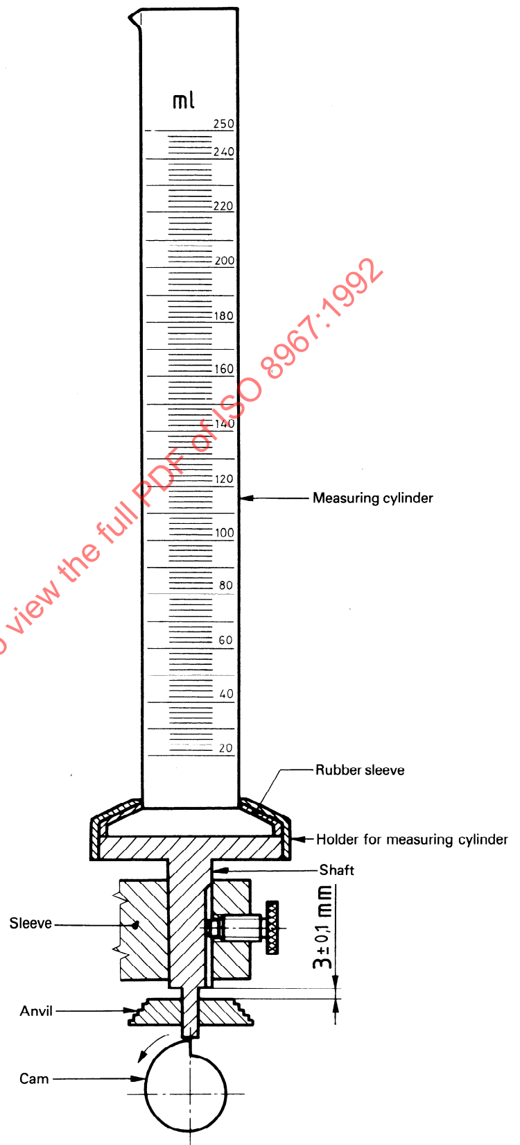
Figure 1 — Bulk density apparatus
