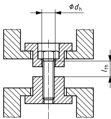
b) Example of testing device for screws
