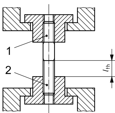
c) Example of testing device for studs
