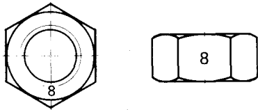
Figure 3 — Examples of marking with designation symbol
