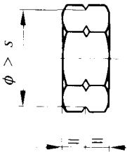
Figure 6 — Alternative left-hand thread marking
