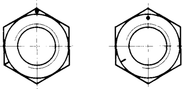
Figure 4 — Examples of marking with code symbol (clock-face system)
