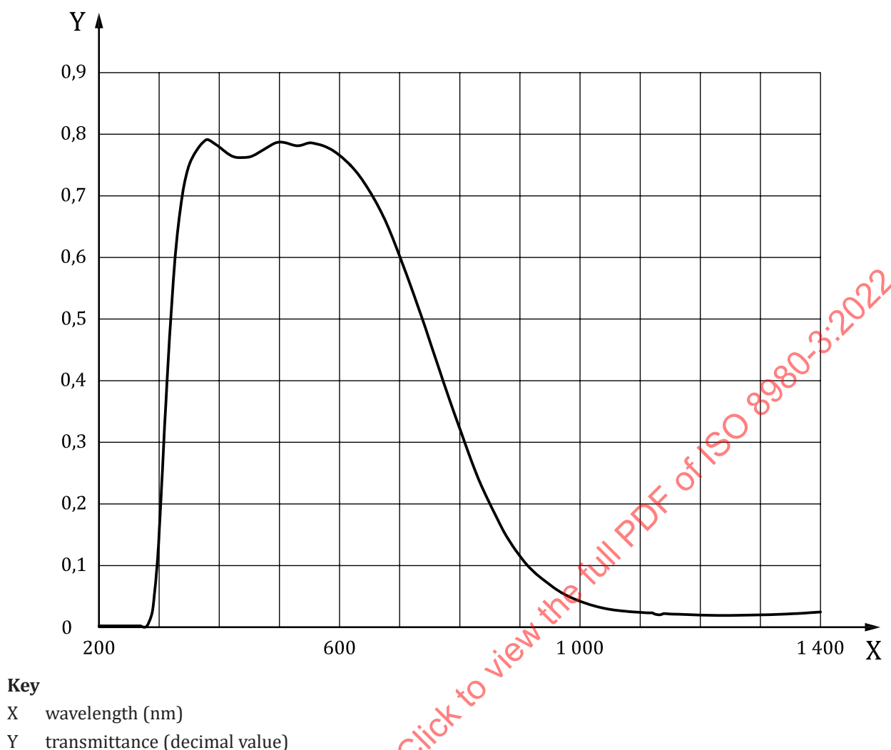
Figure 1 — Spectral transmittance of the combination of the heat absorbing filter and the cut-on filter for the irradiation of photochromic lenses
