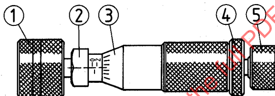
Figure 1 — Volume micrometer
