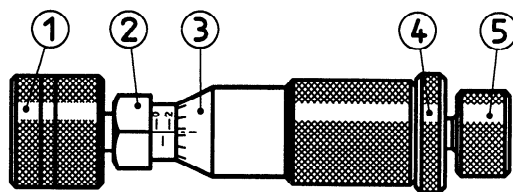
Figure 1 — Volume micrometer
