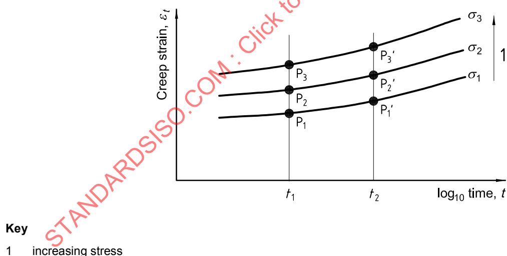
Figure 1 — Creep curves
