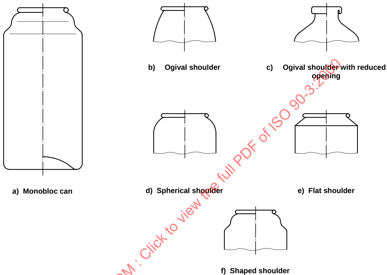
Figure 4 — Monobloc can
