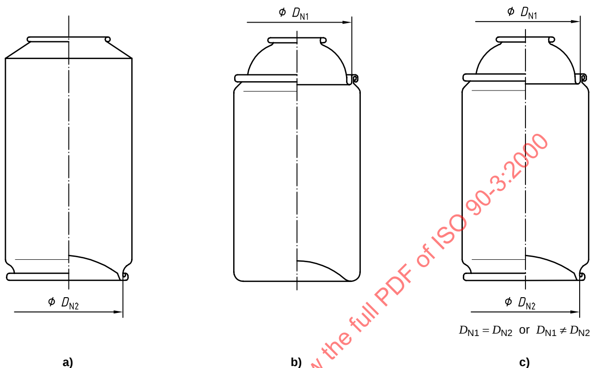
Figure 6 — Necked-in can
