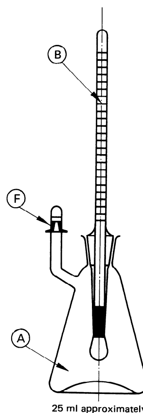
FIGURE 1 — Pyknometer (5.1)
