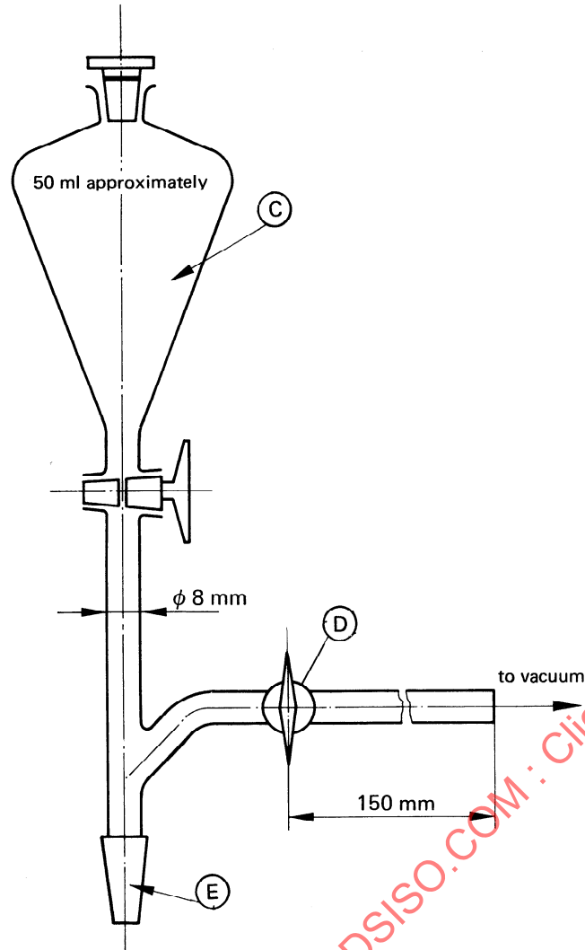
FIGURE 2 — Degassing apparatus (5.2)
