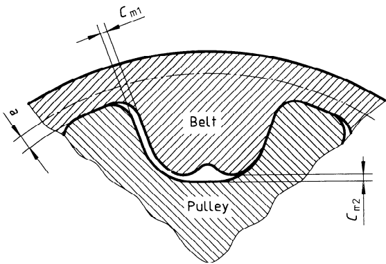
Figure 9 — Clearance between measuring pulley and belt types ZR and YR (see table 10)
