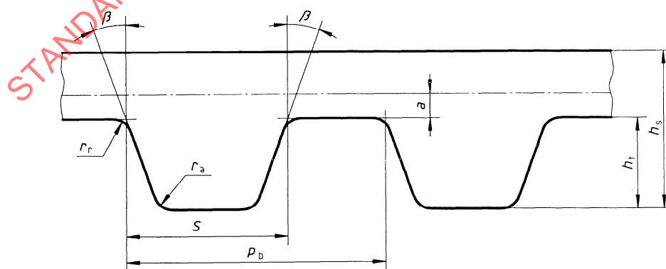
Figure 1 — Nominal tooth dimensions (profile) for types ZA and ZB
