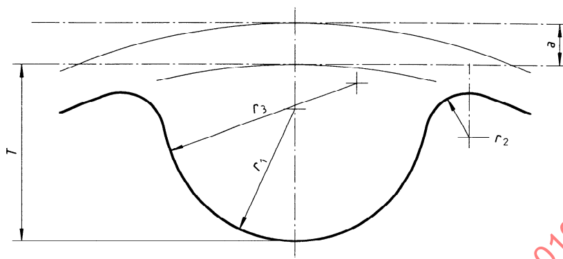
Figure 7 — Measuring pulley grooves for types ZH and YH (see table 9)
