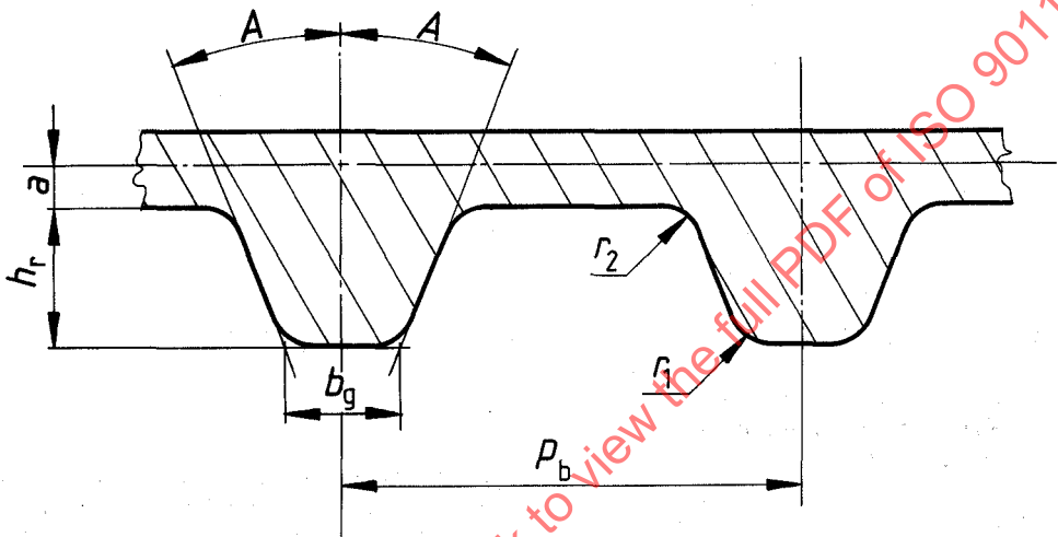
Figure 1 — Generating tool rack for pulleys
