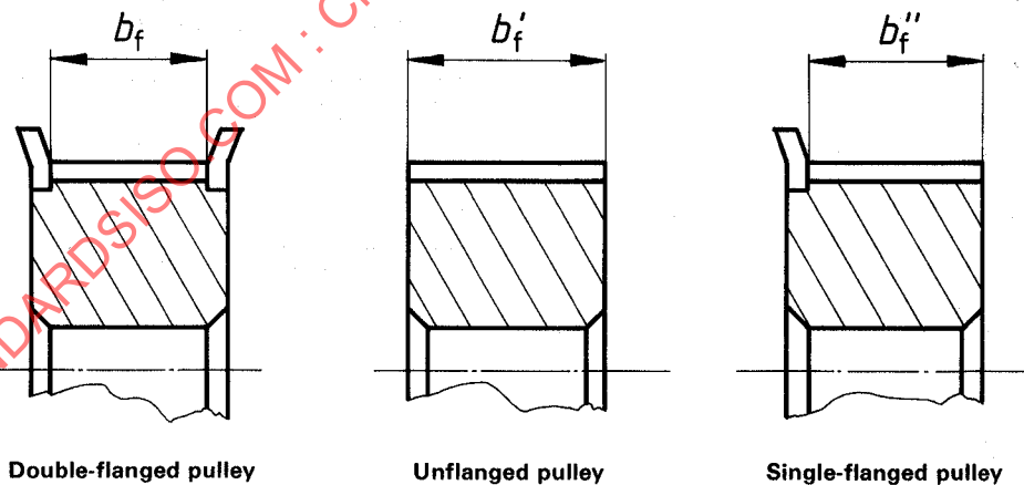
Figure 2 — Minimum pulley width
