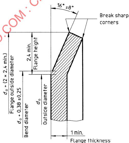
Figure 8 — Flange dimensions
