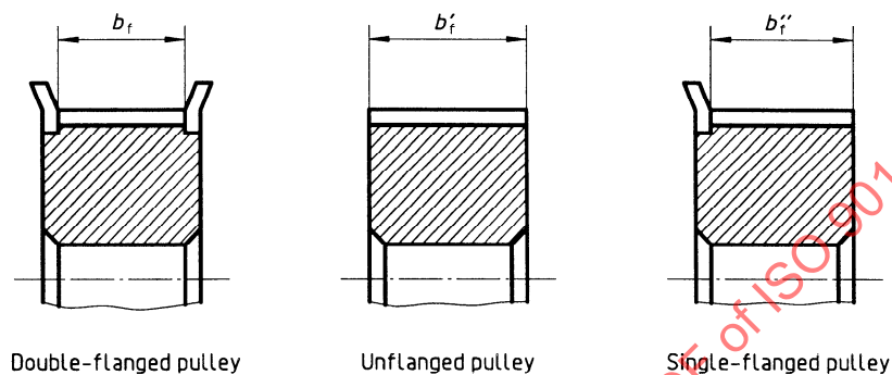
Figure 7 — Minimum pulley width
