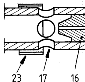
Figure 1 — Schematic drawing of the mixing zone
