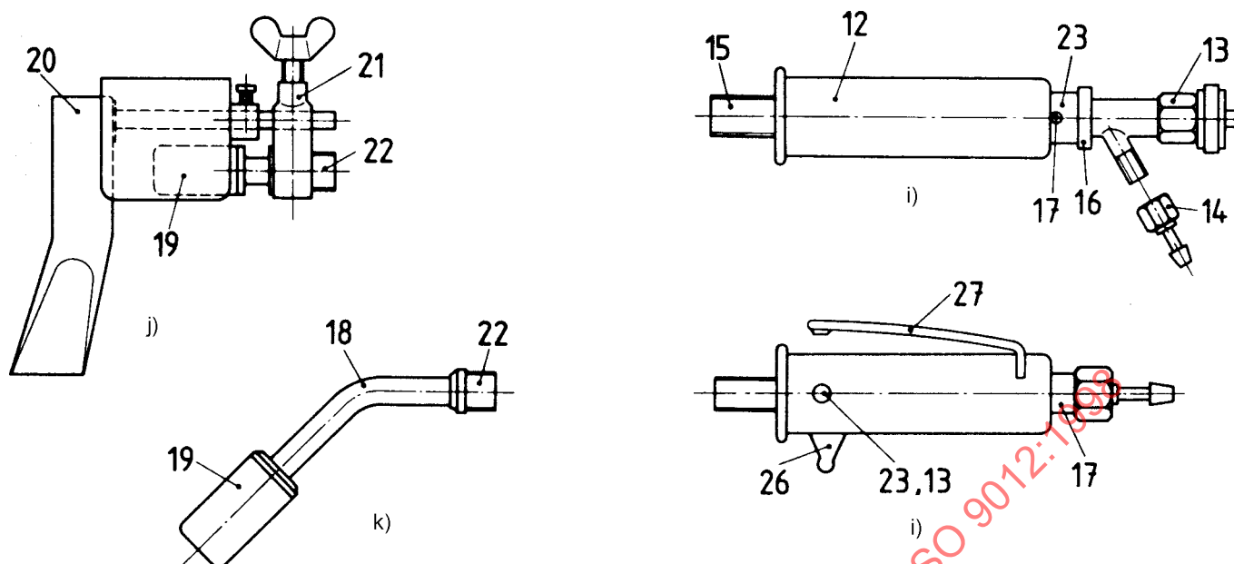
Figure 4 — Examples of blowpipes with air aspiration in the shank
