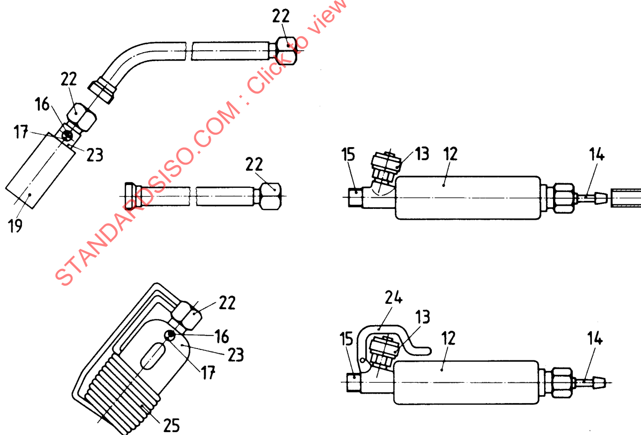
Figure 2 — Examples of blowpipes with air aspiration in the attachment
