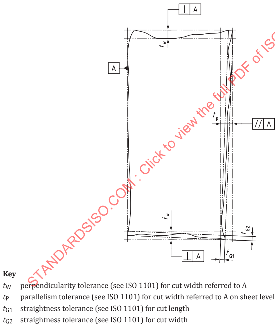
Figure 11 — Form and location tolerances shown by the example of a sheet plate
