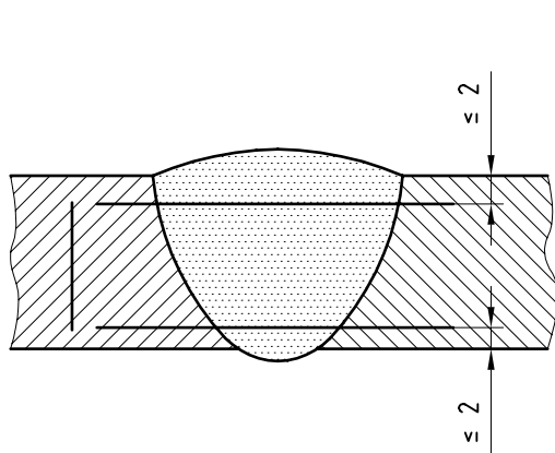
a) Butt weld from one side only both single and multirun
