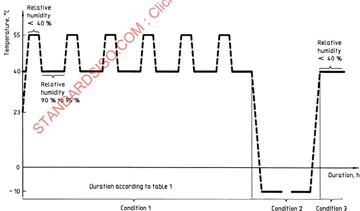
Figure 1 — Cycling curve for conditioning method 47, using example of degree of severity 01
