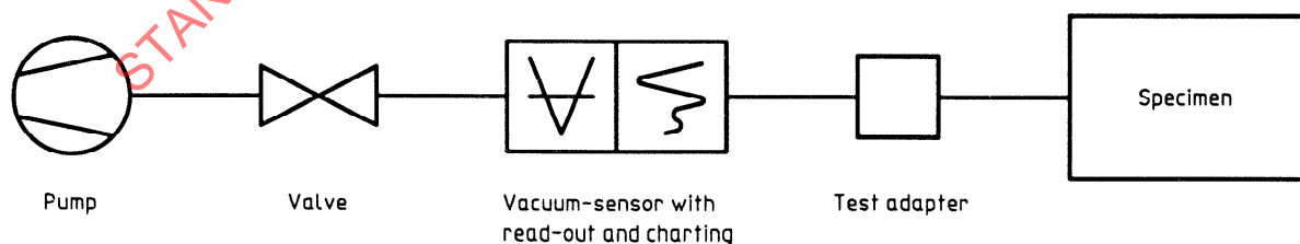
Figure A.1 — Schematic representation of pressure test apparatus suitable for test methods 80 and 81
