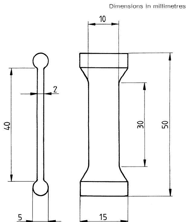
Figure 4 — Dumb-bell test piece with beaded ends
