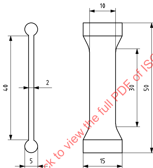
Figure 4 — Dumbbell test piece with beaded ends
