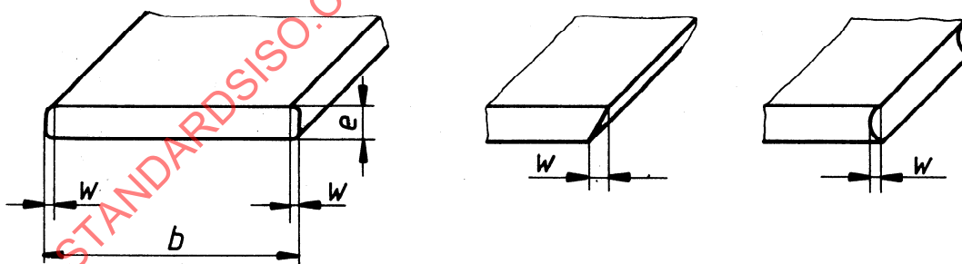
Figure 1 — Angular accuracy
