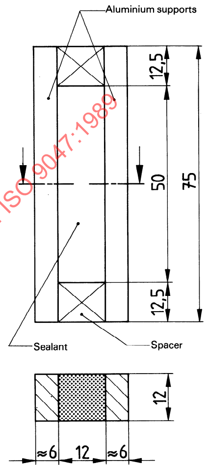
Figure 2 — Test specimen with aluminium supports
