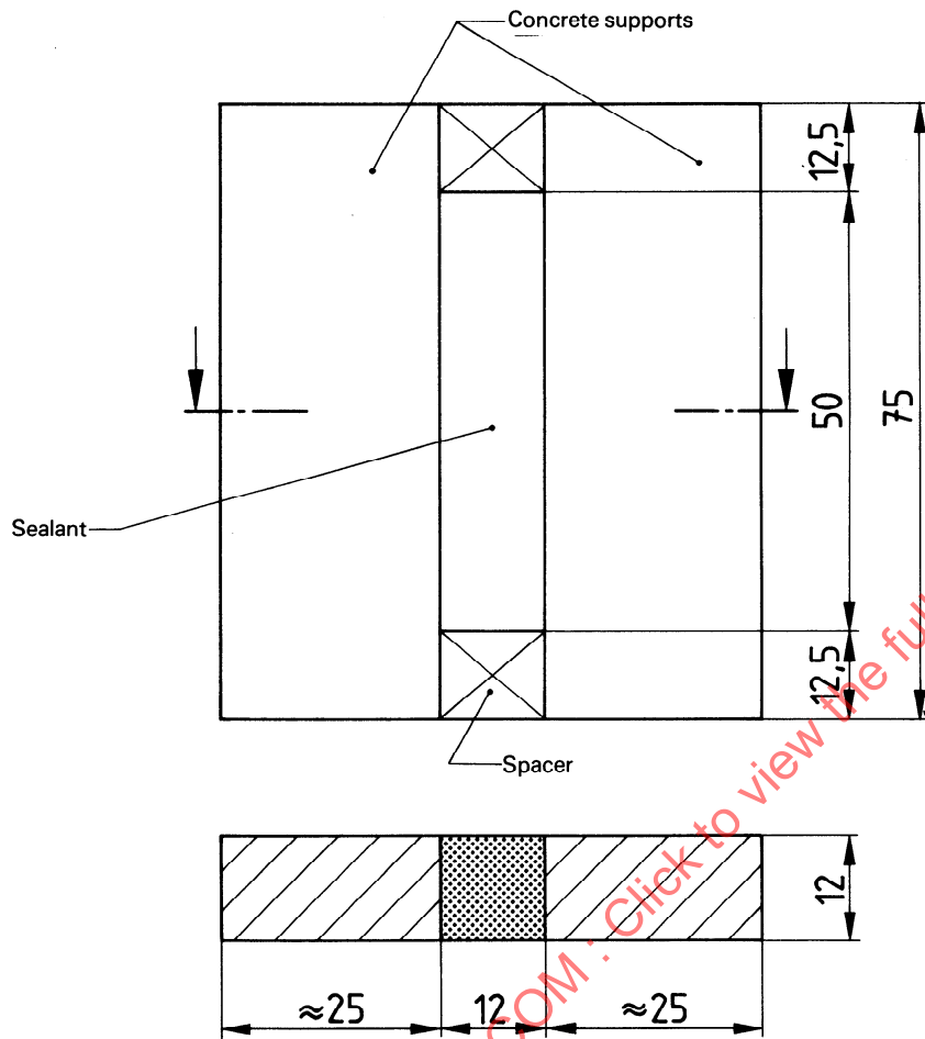
Figure 1 — Test specimen with concrete supports
