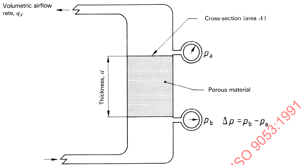
Figure 1 — Direct airflow method (method A) — Basic principle
