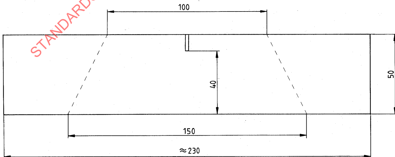
Figure 1 — Template for trapezoid tearing test
