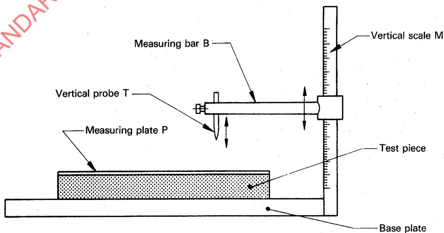
Figure 2 — Test apparatus for bulky nonwovens with a thickness greater than 20 mm
