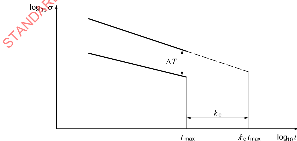
Figure 1 — Extrapolation time in the case of extrapolation without a knee at the highest test temperature
