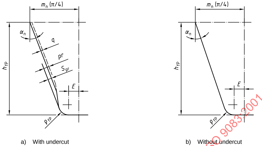
Figure 4 — Dimensions and basic rack profile of teeth (finished profile)
