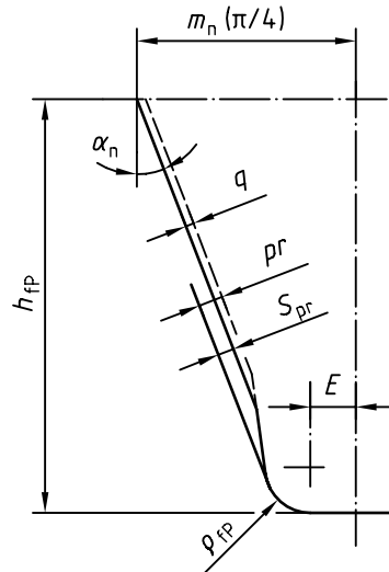
Figure 4 — Basic rack profile of protuberance rack
