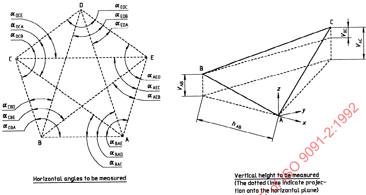
Figure 10 — Data measured for coordinate determination
