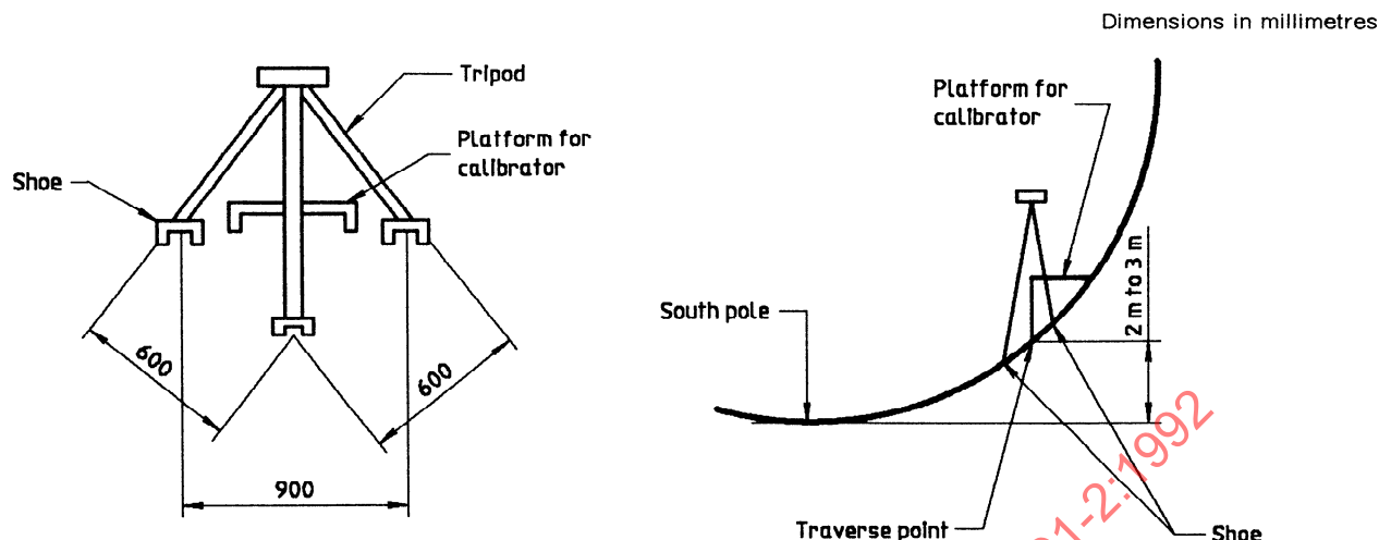
Figure 4 — Example of shoe arrangement for platform
