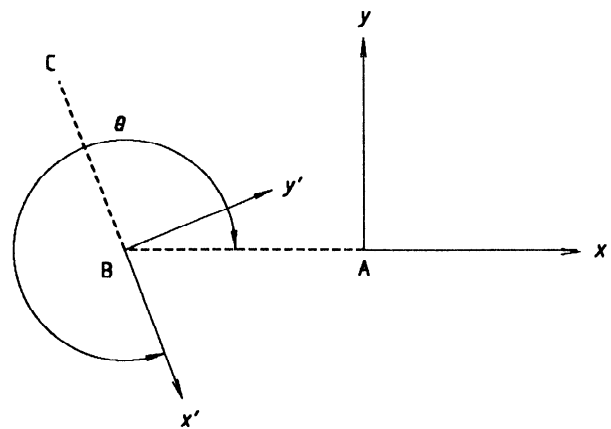
Figure 15 — Transformation from local coordinate ( x' , y' , z' ) system to basic coordinate ( x , y , z ) system
