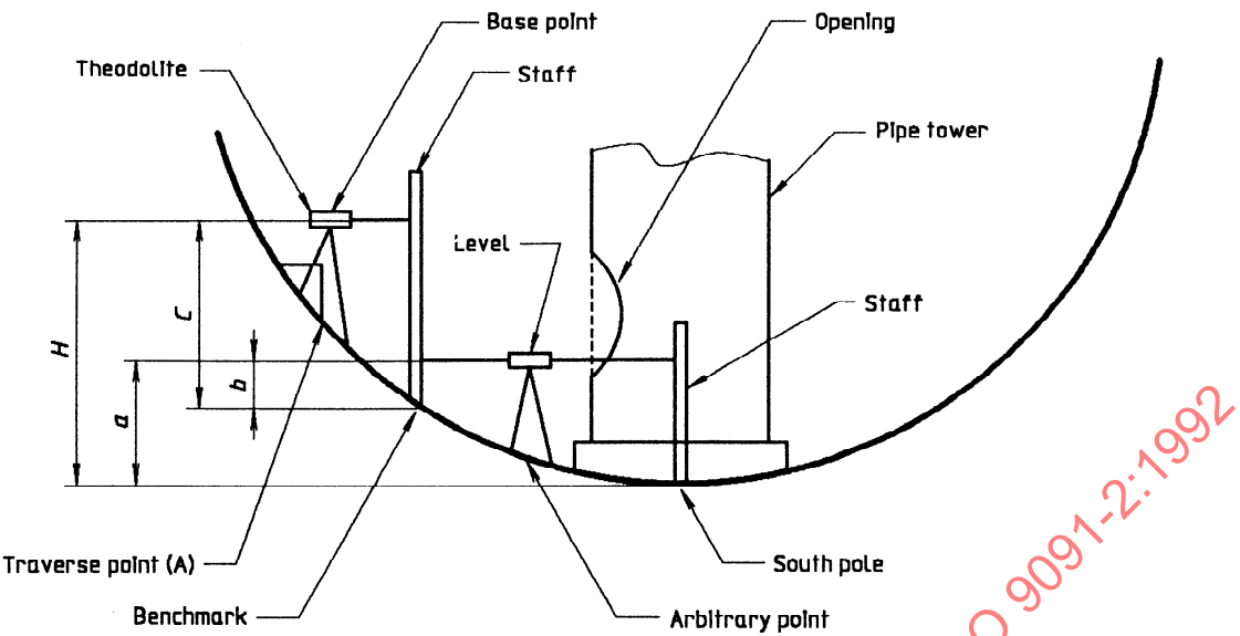
Figure 2 — Set-up of instruments for determining the height of the base point
