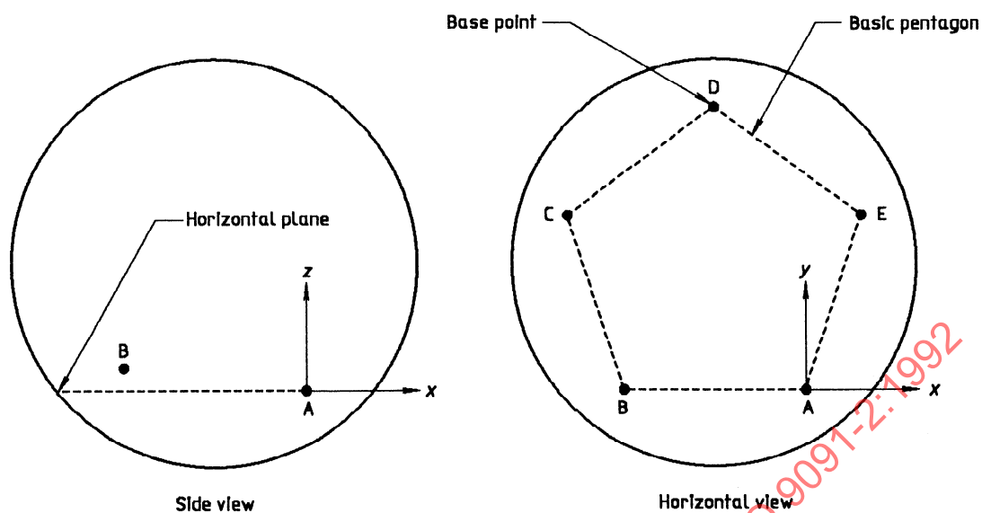
Figure 8 — Coordinate system for calculation
