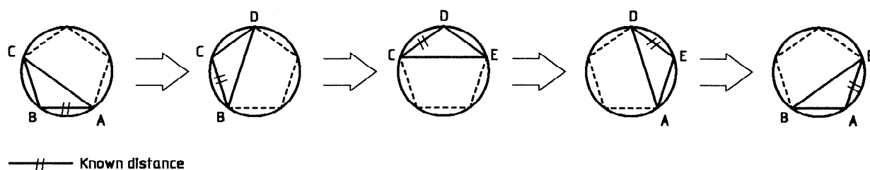
Figure 12 — Calculation order
