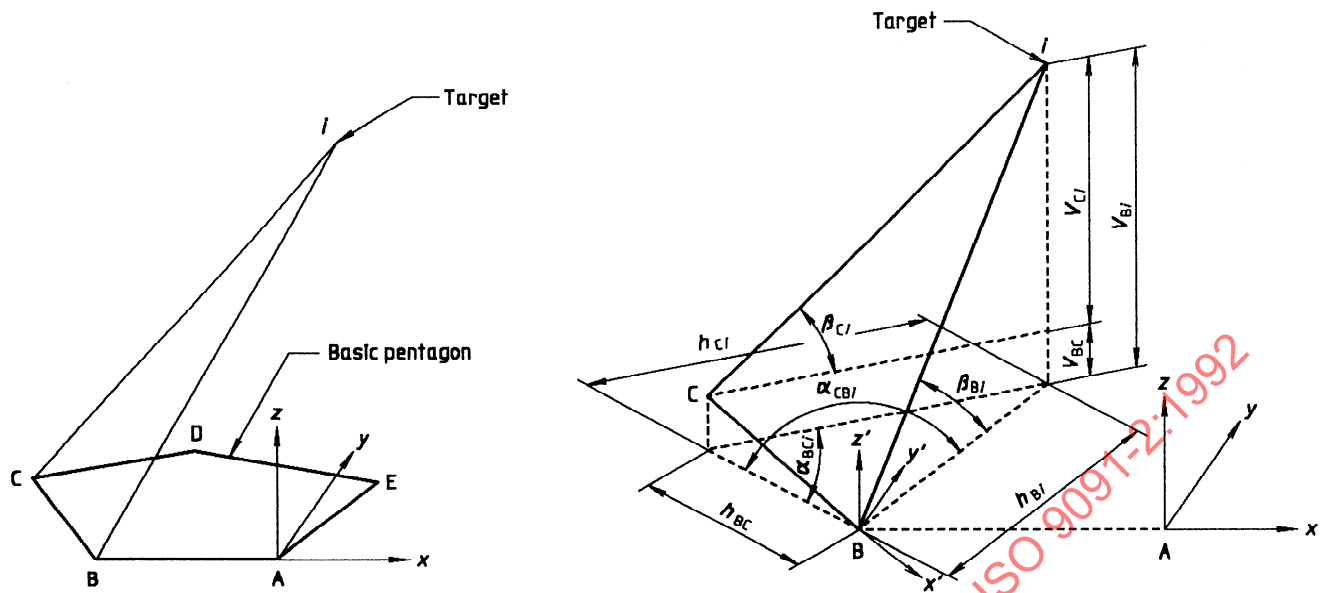
Figure 14 — Coordinates of a target
