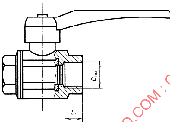
Figure 1 — Seacock
