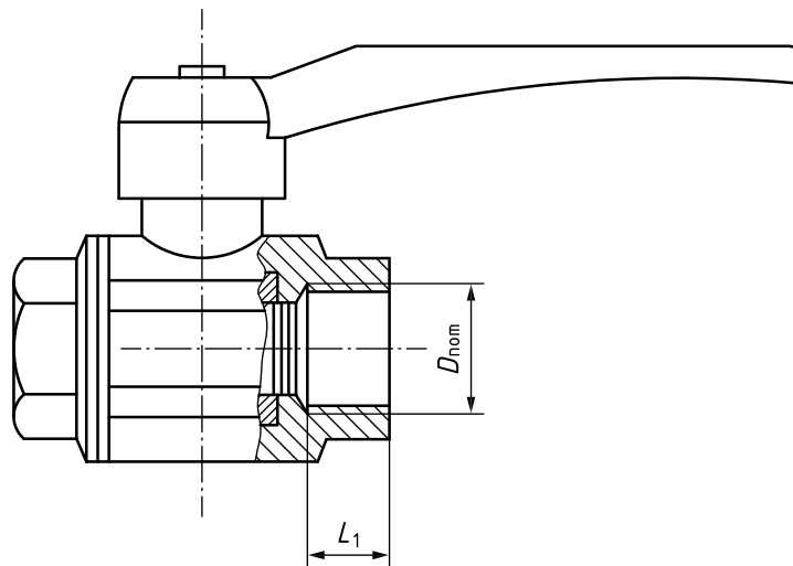
Figure 1 — Seacock
