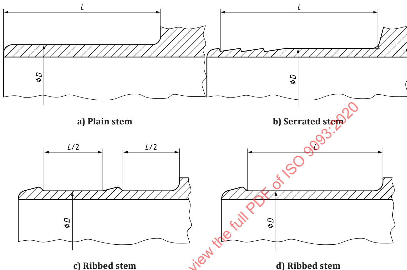
Figure 2 — Examples of hose fittings
