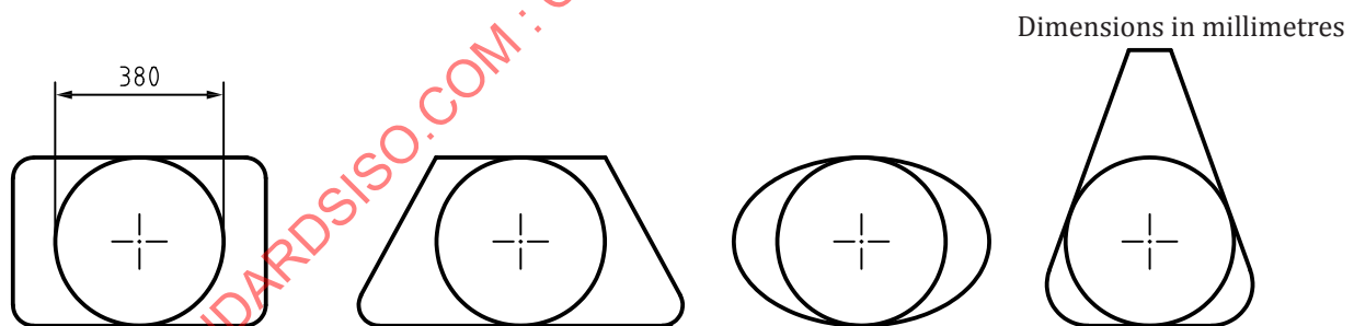
Figure 2 — Measurement of minimum clear opening, in millimetres
