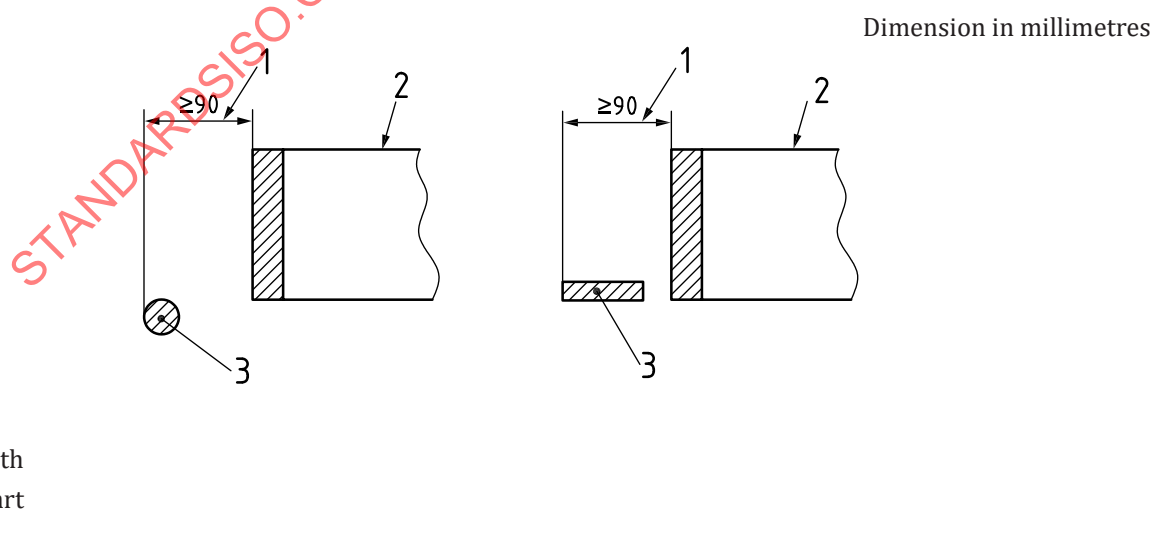
Figure 5 — Gaps and step depth – Example of construction
