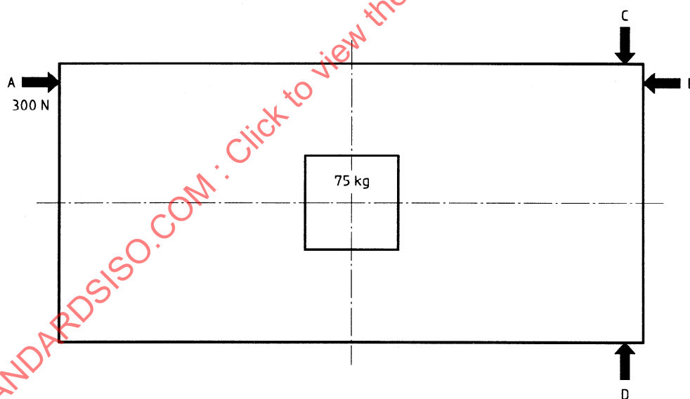
Figure 6 — Application of load and forces
