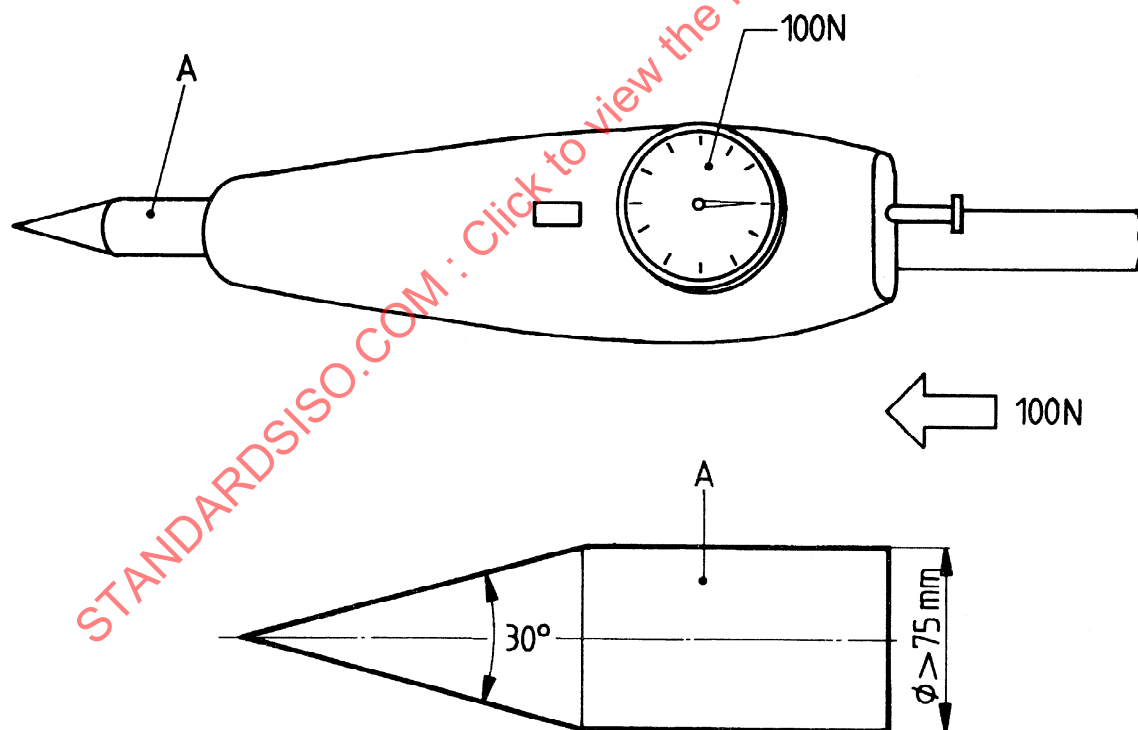
Figure 1 — Example of measuring cone
