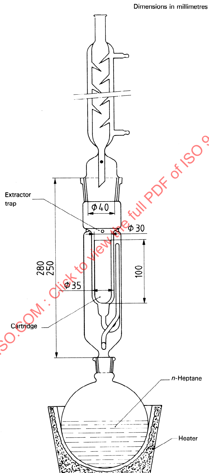
Figure — Extraction apparatus capable of receiving the cartridges described in 3.2
