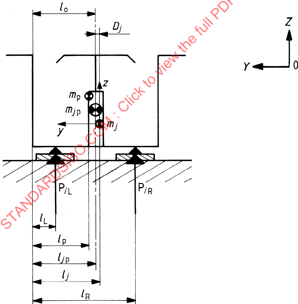
Figure 2 — Measurement procedure for location of centre of gravity along y -axis
