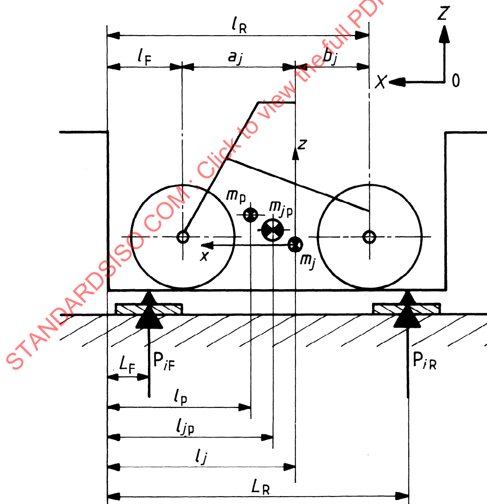
Figure 1 — Measurement procedure for location of centre of gravity along x -axis
