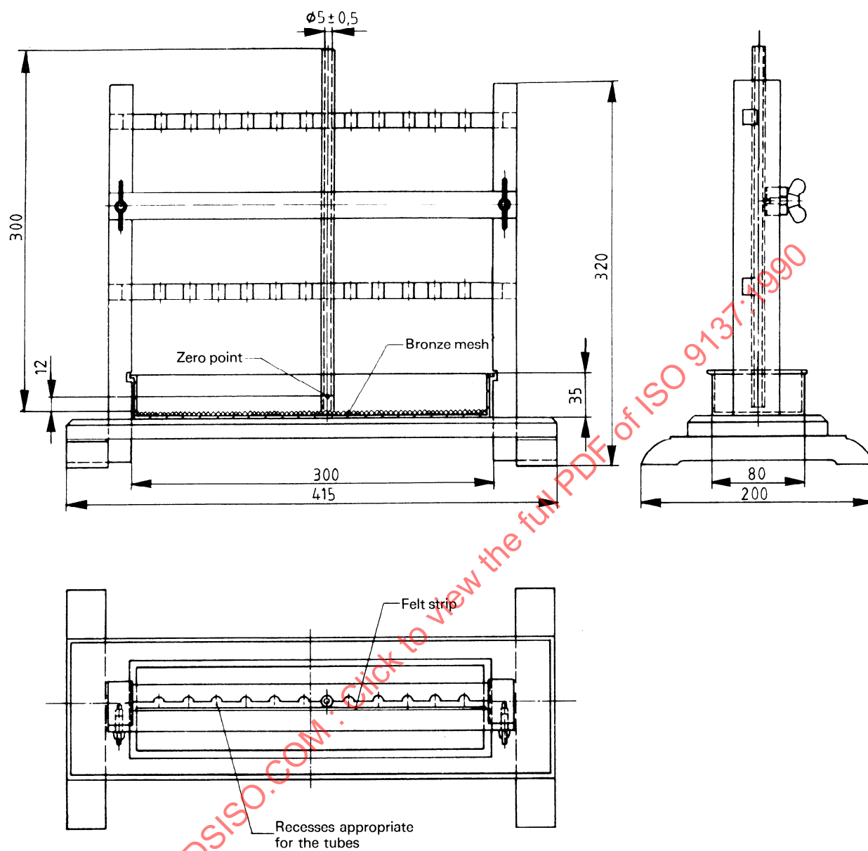
Figure 1 — Possible design of the capillarity measuring apparatus
