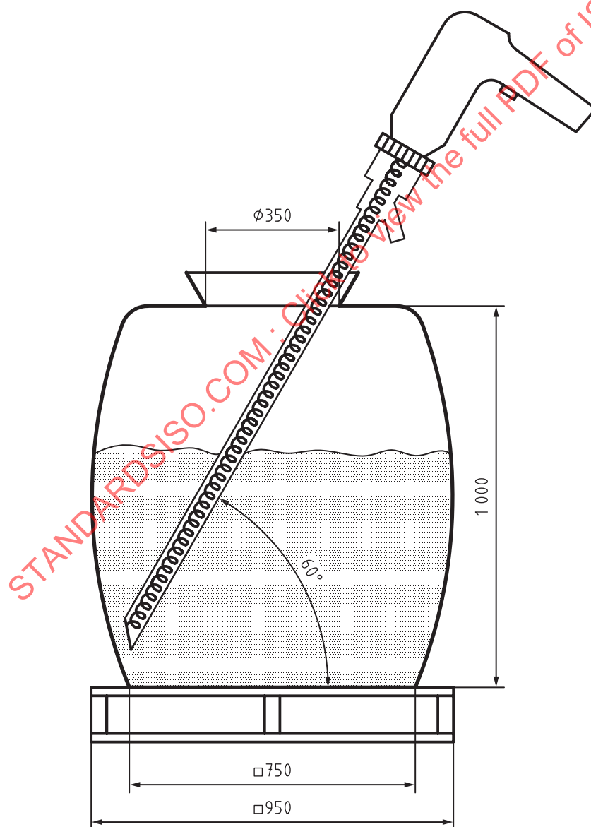
Figure 6 — Sampling big-bags
